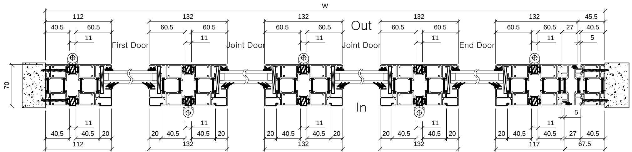
Plan Detail
