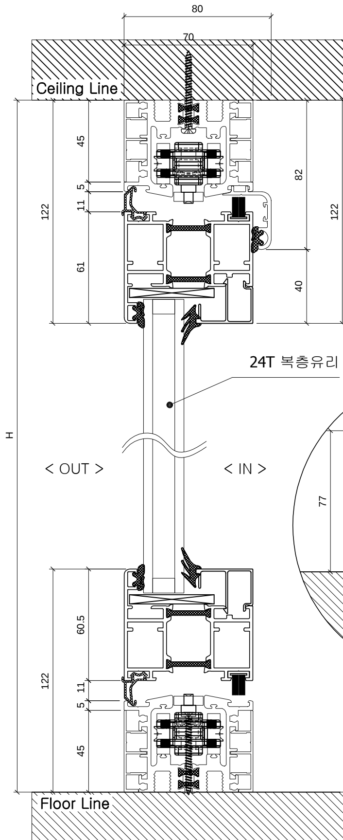
Section Detail
