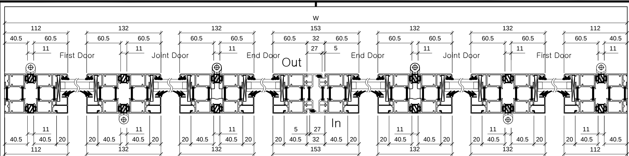
Plan Detail
