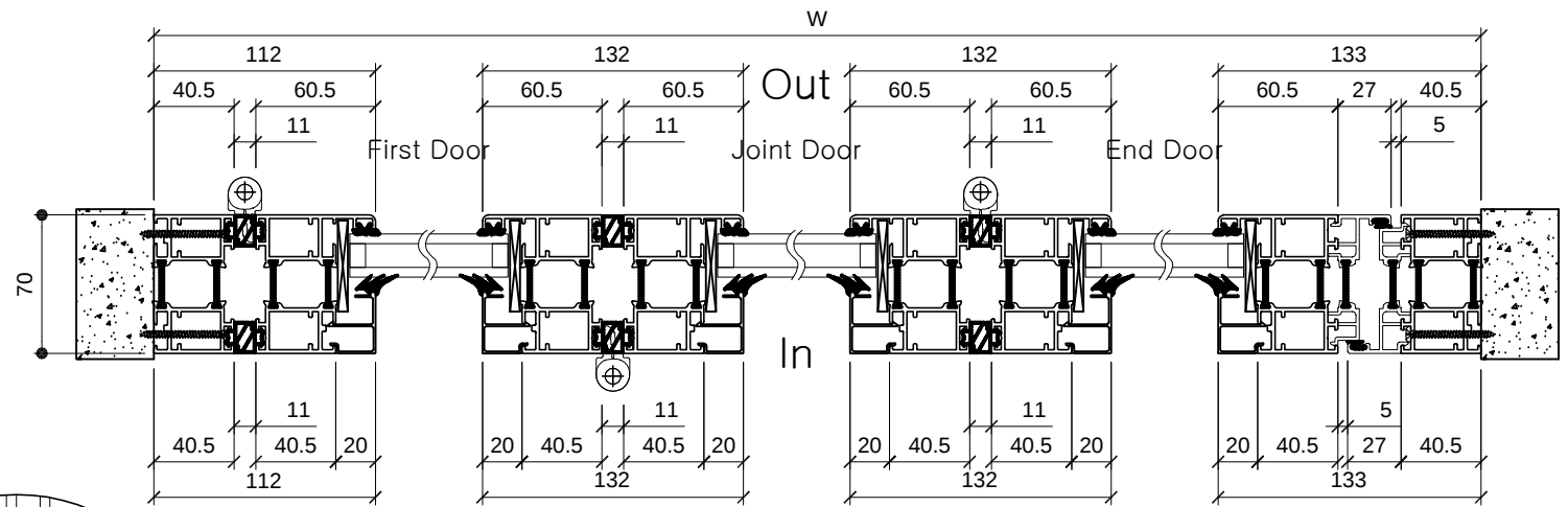
Plan Detail
