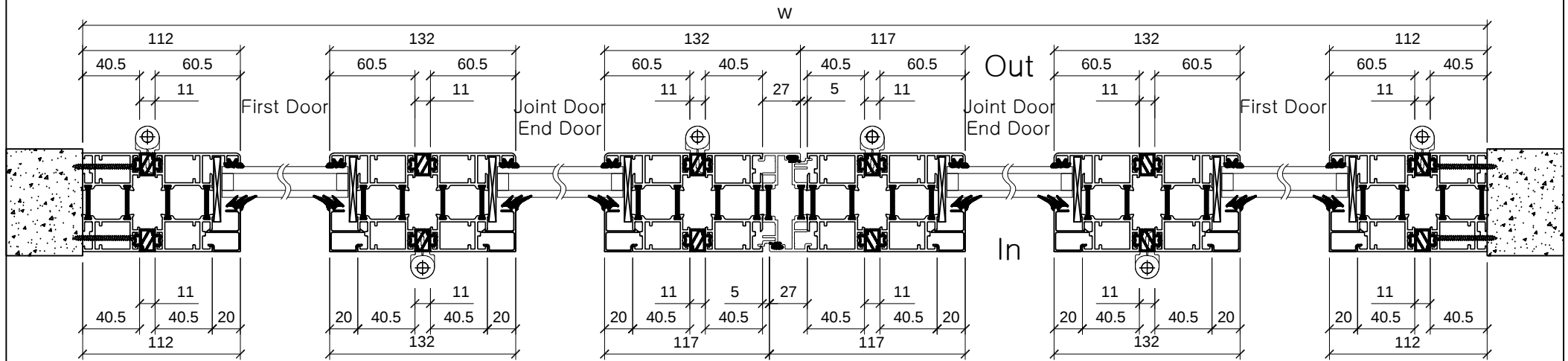
Plan Detail
