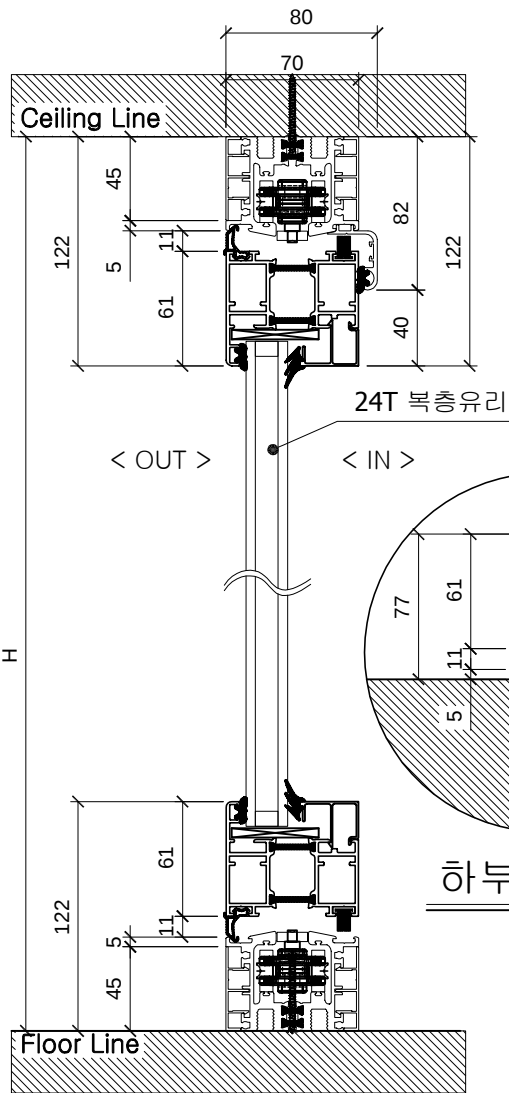
Section Detail
